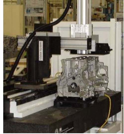
The ERC/RMS Reconfigurable Inspection Machine is inspecting engine blocks on a Chrysler production line in Dundee, Michigan
