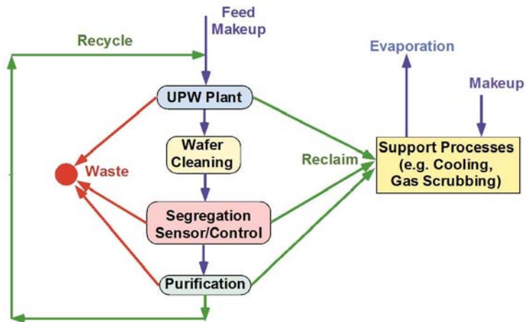
Water Use and Reuse in Semiconductor Manufacturing (Role of Integration in the Design for Environment)
