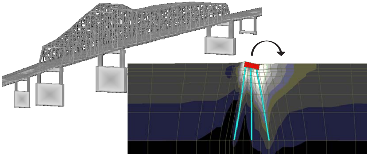
3D simulation model of the Caruthersville bridge including refined soil and deep foundation modeling.
