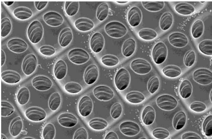
SEM image of crystalline pattern on STAR material surface.
